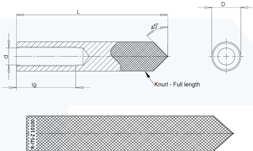
Figure A2 : Anchor rods with inner thread
